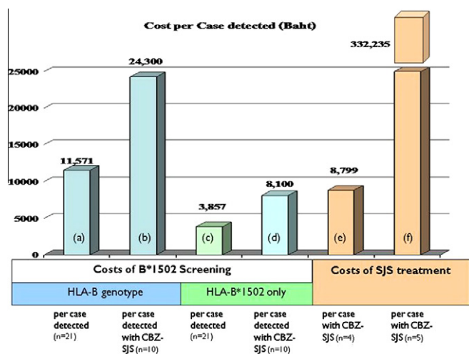
Fig. 2. Cost-effectiveness study of HLA-B*1502 screening to prevent Steven–Johnson syndrome/toxic epidermal necrolysis (SJS/TEN) from carbamazepine showing: (a) and (b) compared to (e) that the costs of HLA-B*1502 screening per case detected will exceed those of SJS treatment when a polymerase chain reaction-based HLA-B genotyping kit was used; whereas (c) and (d) compared to (e), screening costs will be less than SJS treatment if a HLA-B*1502 -specific test is used. (f) The cost of SJS treatment per case, which included one patient who had an unusually prolonged hospitalization. (This figure is available in colour at www.sciencedirect.com .)
