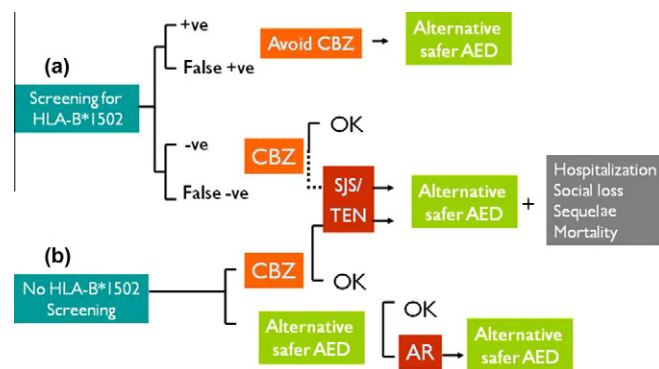
Fig. 1. Schematic of strategies in evaluating cost effectiveness of blood screening for the HLA-B*1502 allele prior to prescribing carbamazepine (CBZ) in an outpatient epilepsy setting showing that (a) screening for HLA-B*1502 can prevent the possible Steven–Johnson syndrome/toxic epidermal necrolysis (SJS/TEN) by avoiding CBZ in test-positive individuals, but may be misleading in 5% to 19% of patients who are false positive; in contrast, in most patients who are HLA-B*1502 negative, CBZ can be used rather safely since the negative predictive value is very high (98%); and (b) without HLA-B*1502 screening, there is low risk of developing SJS/TEN that may increase medical costs, social loss as well as morbidity and mortality, but without HLA-B*1502 screening, alternative safer antiepileptic drug (AED) can be used. This strategy may cost more, or still carries a risk of hypersensitivity or adverse reactions (AR), depending on which AED is used. (This figure is available in colour at www.sciencedirect.com .)
